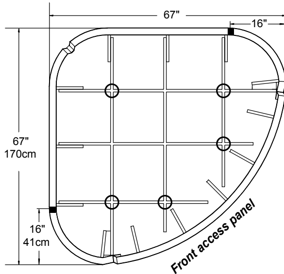
UPSIDE DOWN VIEW OF SPA WITHOUT BASE PAN
